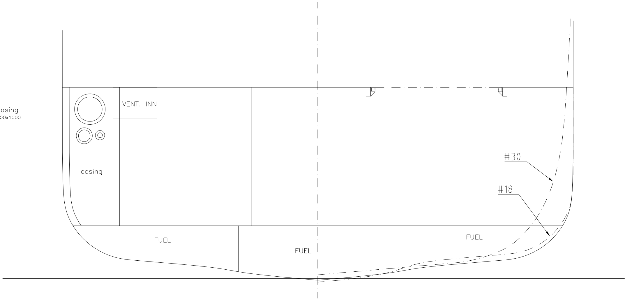
Spant 21
