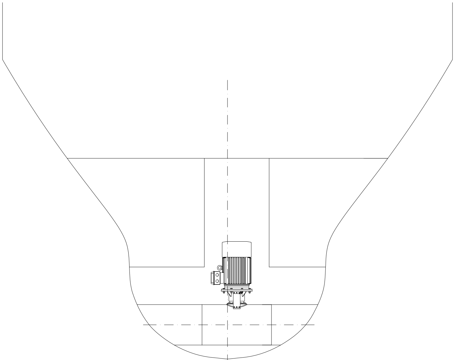
Spant 43
